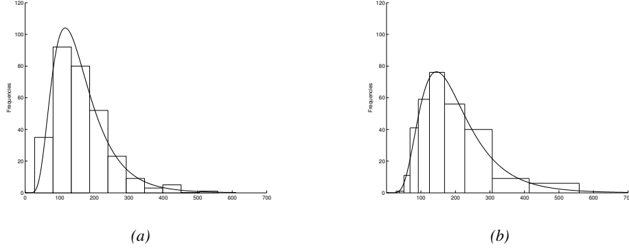
Figure 3: Simulated sample, n = 300 . (a) Histogram and fitted lognormal density; the Lebesgue-lengths of the bins are equal. (b) Display analogous to a histogram and fitted normal in \mathbb{R}_+ density; the \lambda_+ -lengths of the bins are equal.
