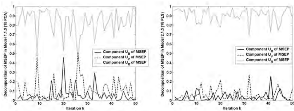
Figure 5: Decomposition of MSEP_i -i = 1, 2, \dots, 50- , for Model 1.1.3 (15 PCA) and Model 2.1.3 (15 PLS).
