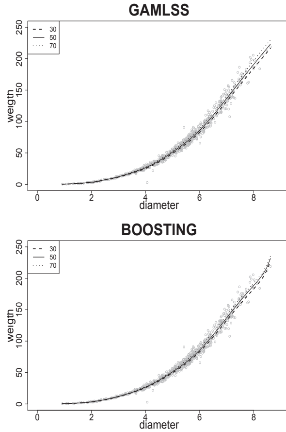
Figure 4: Global population: depiction of the fits for the \tau^{th} percentiles ( \tau \in \{30, 50, 70\} ) with the GAMLSS and BOOSTING techniques.
