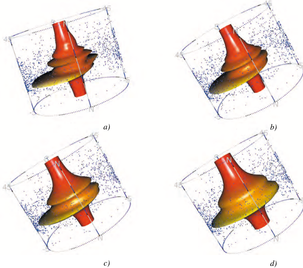
Figure 4: The nonparametric density estimator using different numbers of neighbours, a) k = 75 , b) k = 150 , c) k = 300 and d) k = 400 .
